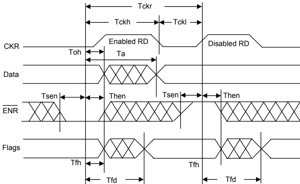
Figure 2: Read Timing
