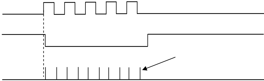
Pre-Charge Pulses on the Data Output pins - Memory Data is all “0s”.
